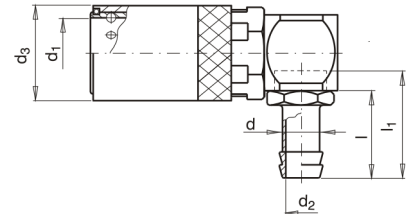
With valve
