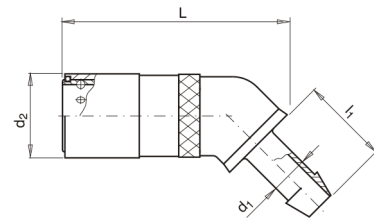
Without valve
